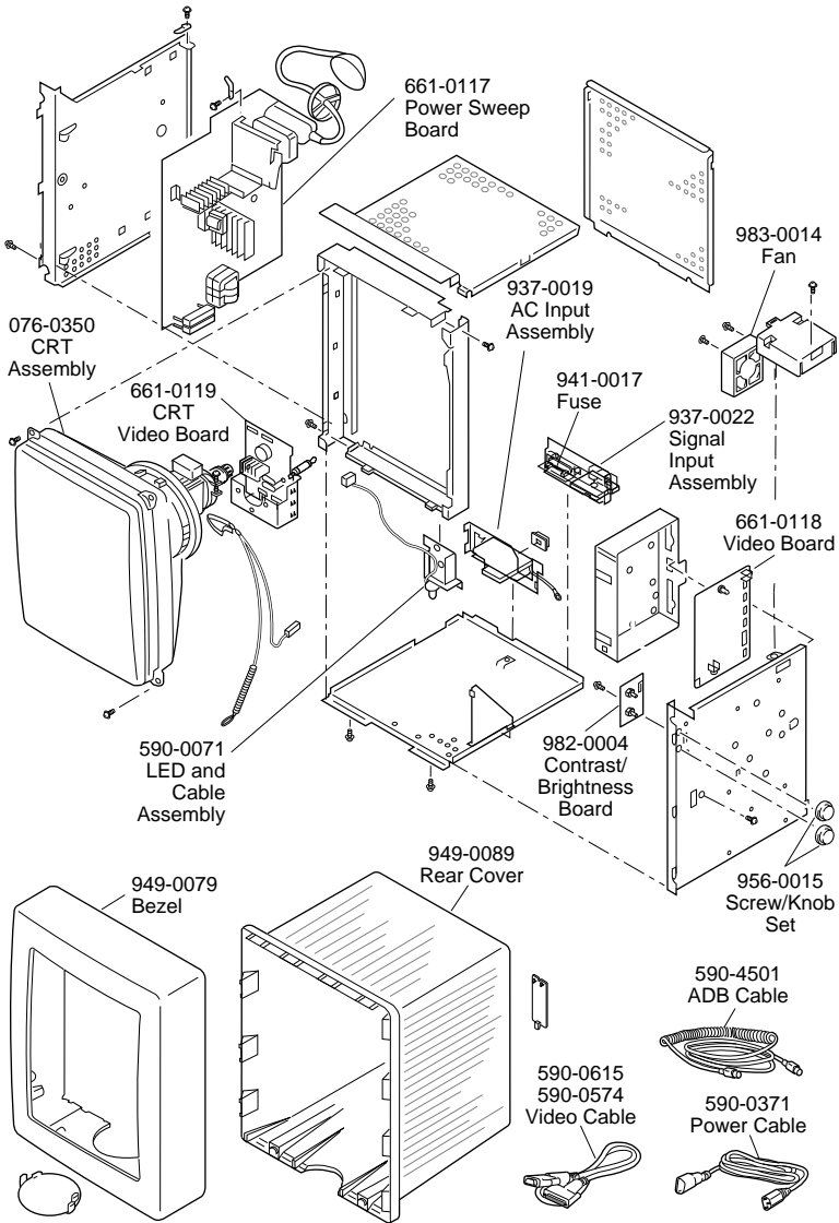
Figure 77. Macintosh Portrait Display Exploded View
